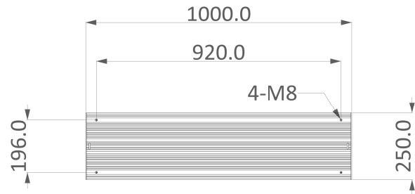
Back view
